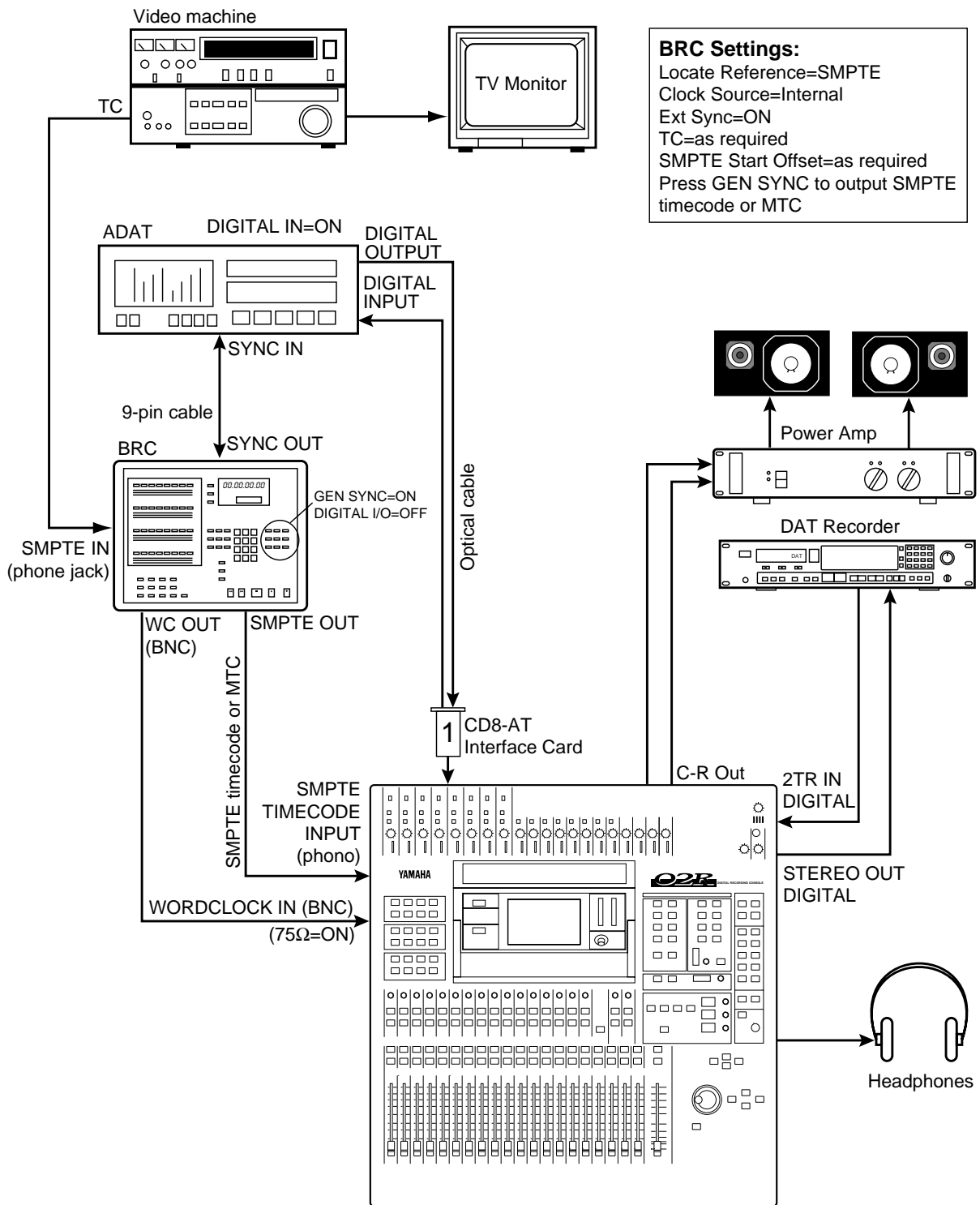
Figure 16 02R with Video Machine, ADAT, & BRC
