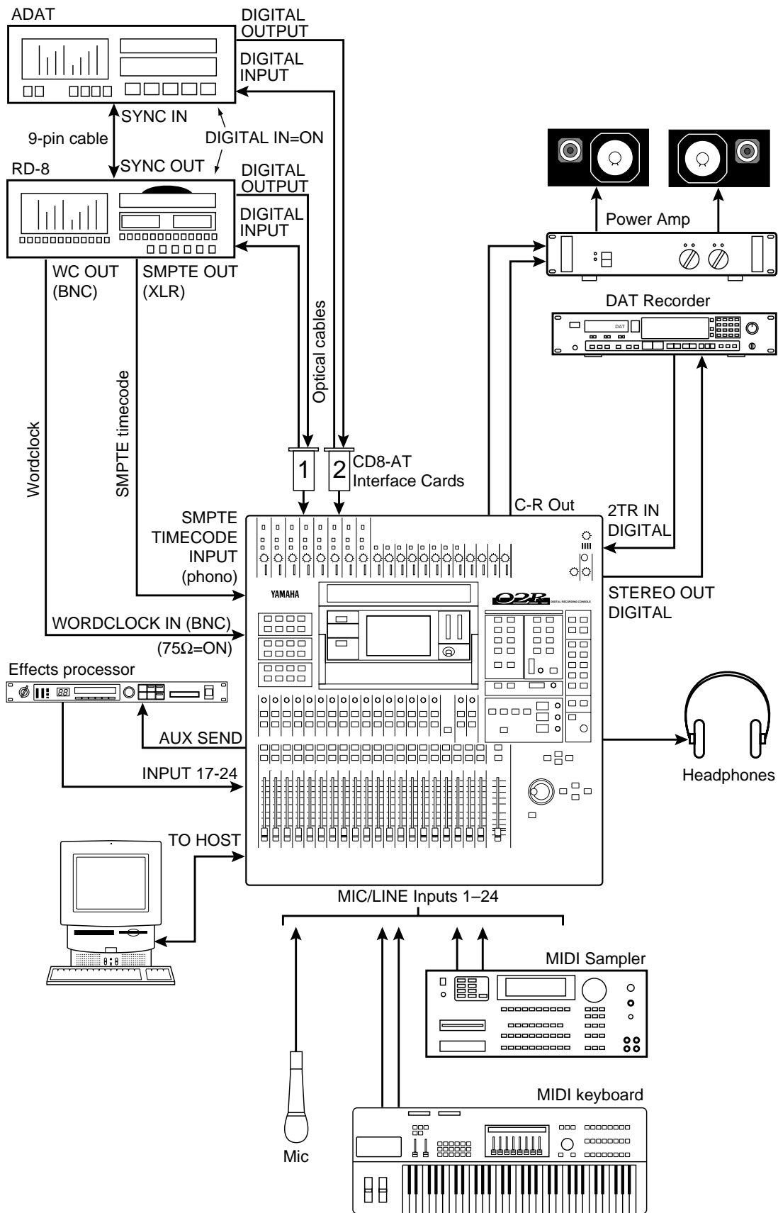
Figure 8 02R with ADAT & RD-8
