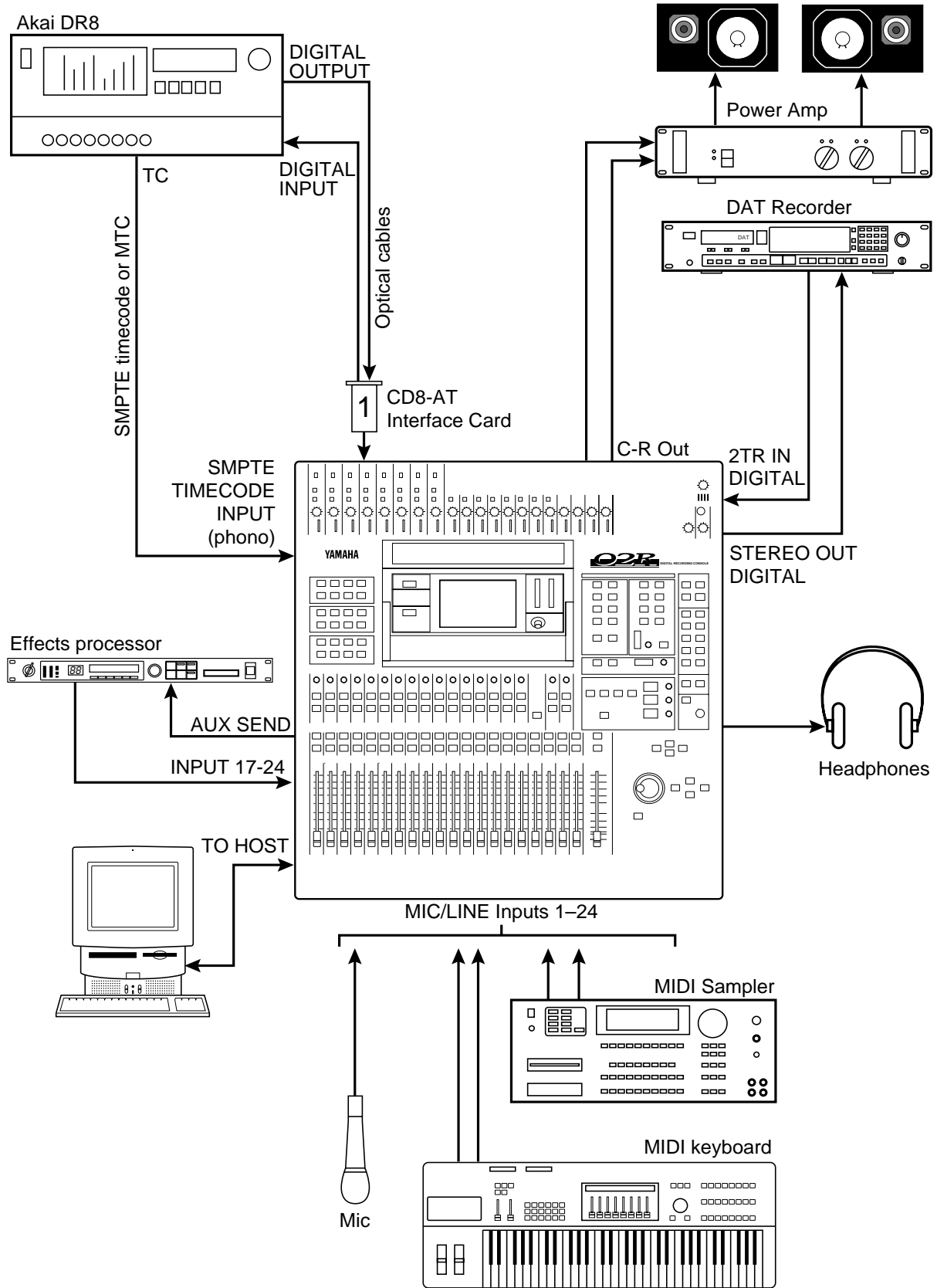
Figure 13 O2R with Akai DR8 Hard Disk Recorder
