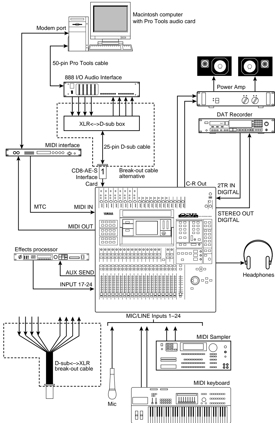
Figure 20 02R with Pro Tools for Music Recording
