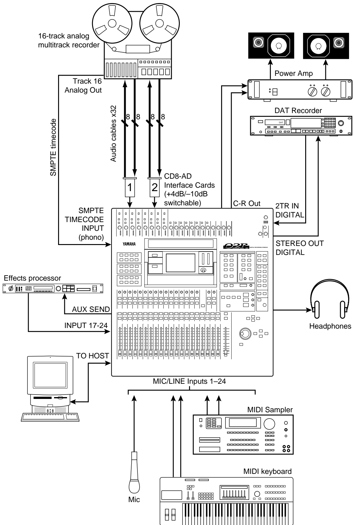
Figure 15 O2R with Analog 16-Track Multitrack Recorder
