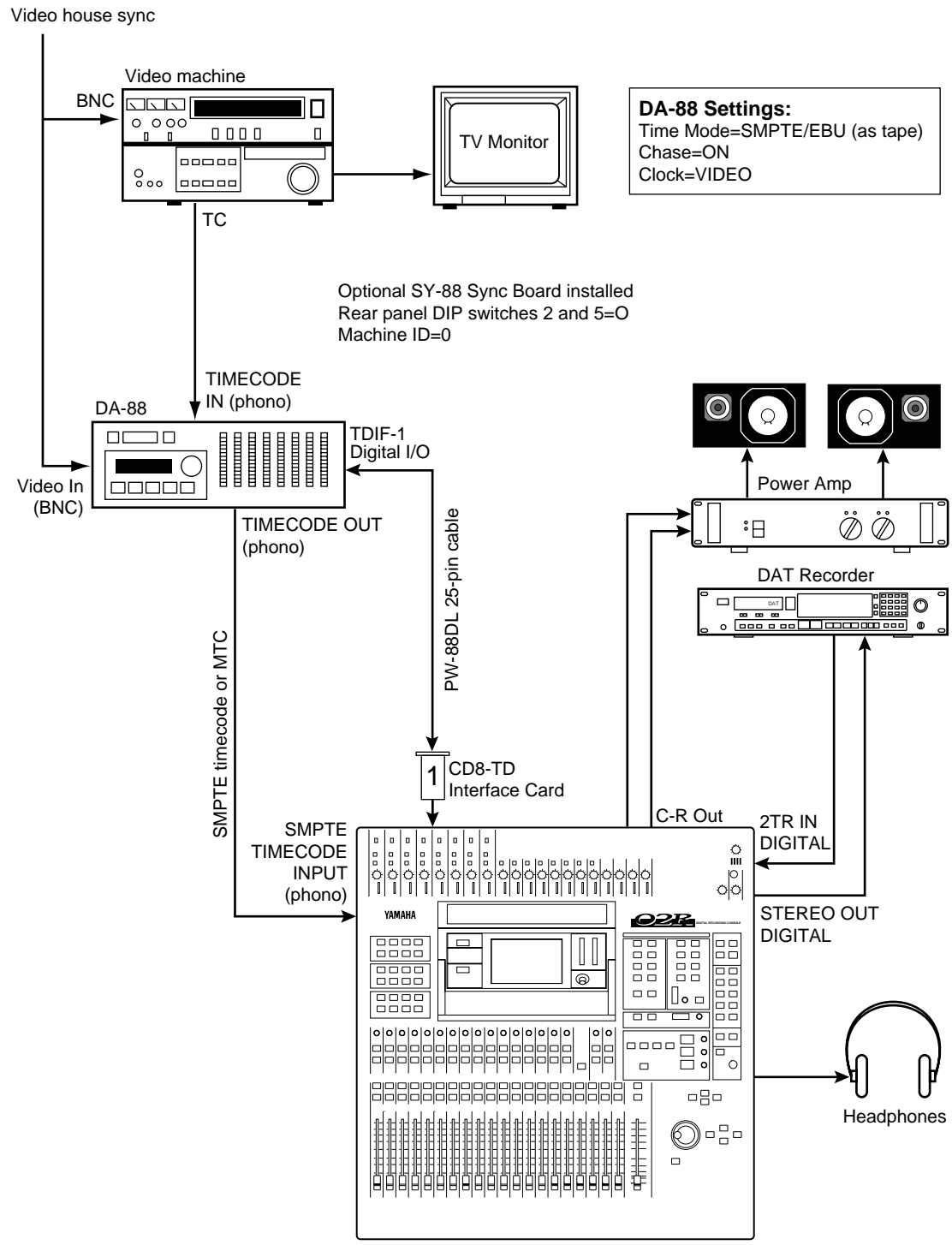
Figure 18 O2R with Video Machine & DA-88
