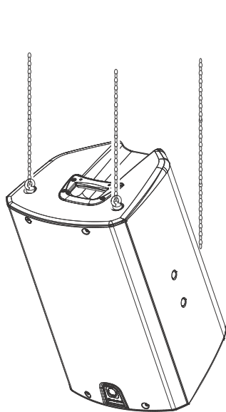
Suspension using M10 shoulder eyebolts.
