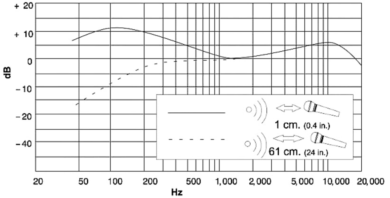
TYPICAL WH30 FREQUENCY RESPONSE
