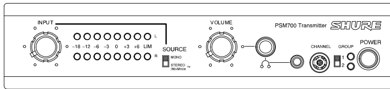
P7T Transmitter with rack-mounting hardware and detachable PA715 antenna
