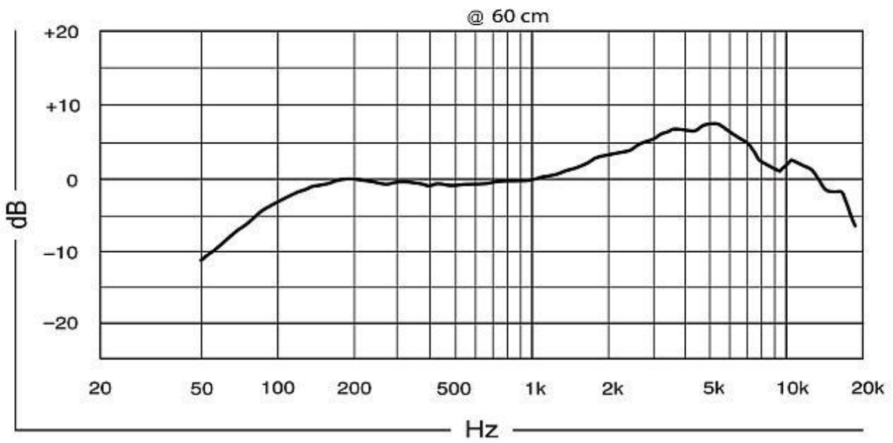
Frequency Response
