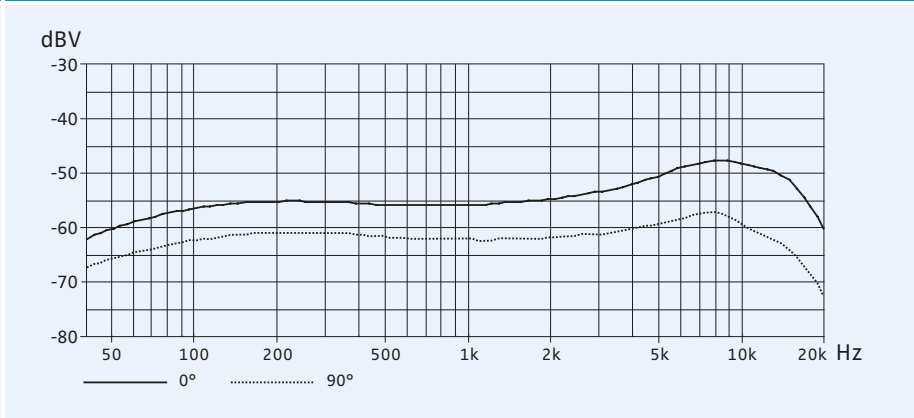
Frequency response curve MME 865-1
