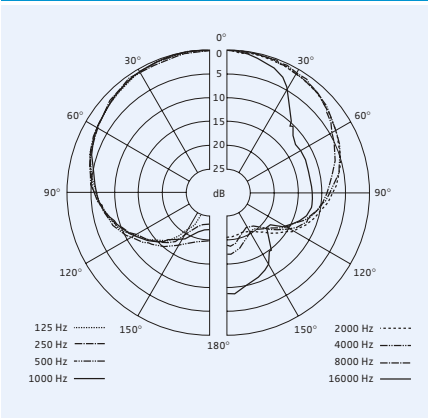
Polar diagram MME 865-1
