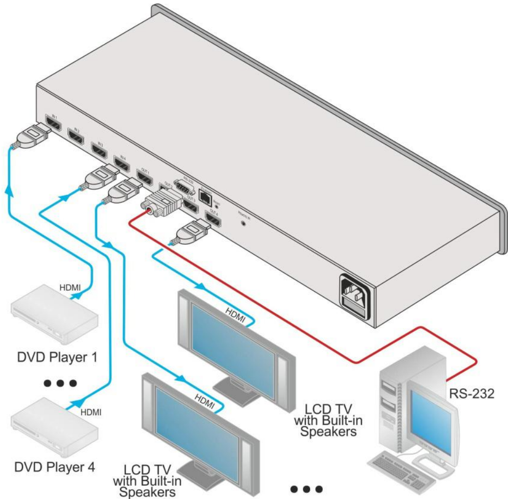
Figure 3: Connecting the VS-44HN 4x4 HDMI Matrix Switcher
