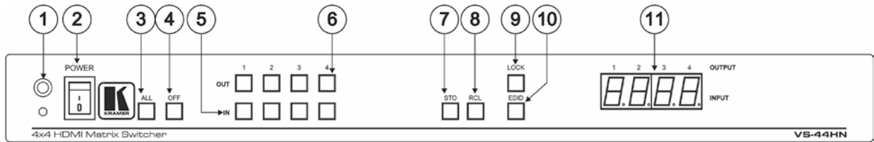
Figure 1: VS-44HN 4x4 HDMI Matrix Switcher Front Panel
