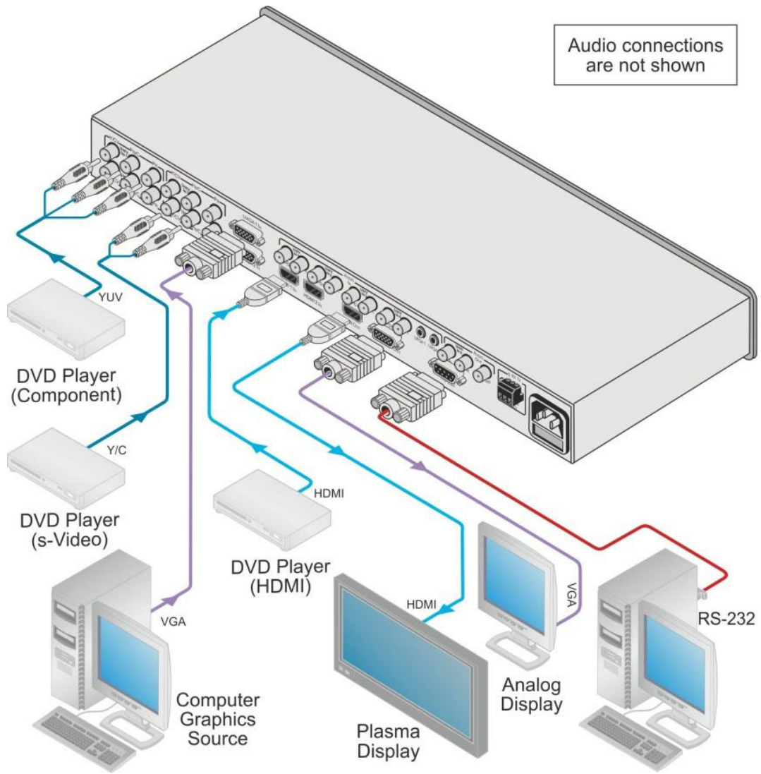
Figure 3: Connecting to the VP-728 Rear Panel
