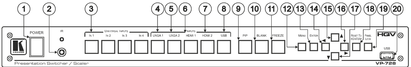
Figure 1: VP-728 Presentation Switcher/Scaler Front Panel
