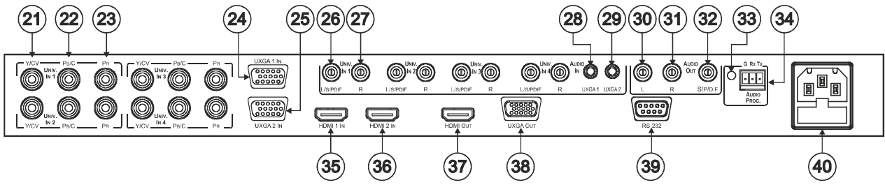
Figure 2: VP-728 Presentation Switcher/Scaler Rear Panel
