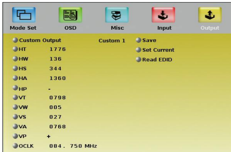
Figure 20: Output Functions
