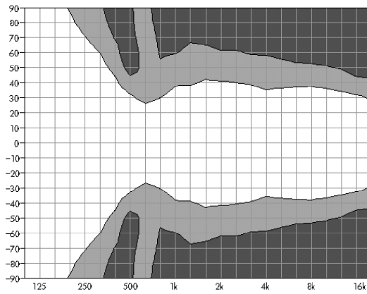
Fig. 7: Isobar diagram Q7 horizontal, horizontal set up with the horn rotated
