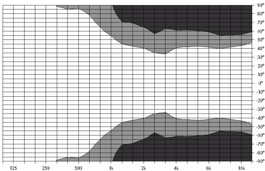
Fig. 7: Isobar diagram E8 horizontal, standard setup
