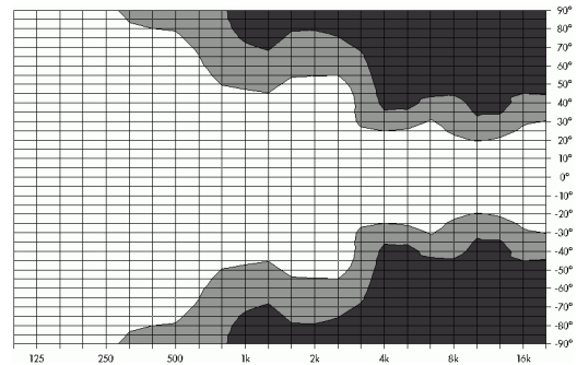
Fig. 8: Isobar diagram E8 vertical, standard setup
