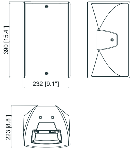
Fig. 12: E8 cabinet dimensions in mm [inch]
