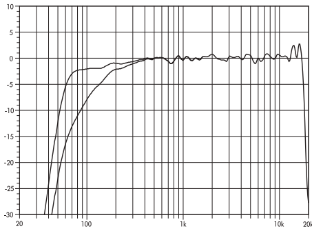
Fig. 11: E8 frequency response, standard and CUT settings
