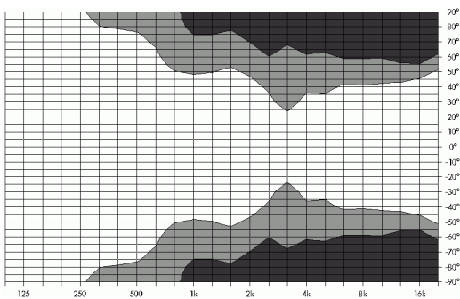
Fig. 9: Isobar diagram E8 horizontal, horizontal setup with the horn rotated
