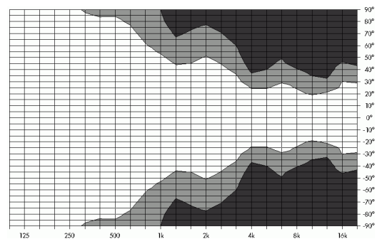
Fig. 10: Isobar diagram E8 vertical, horizontal setup with the horn rotated
