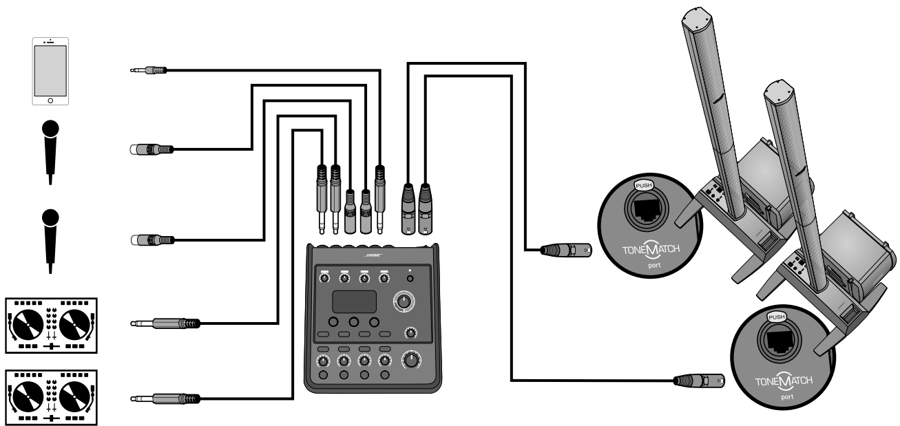
Figure 17. Example setup for stereo DJ/Playback
