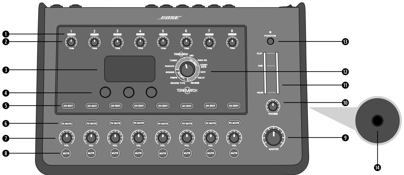
Figure 3. T8S Control Panel
