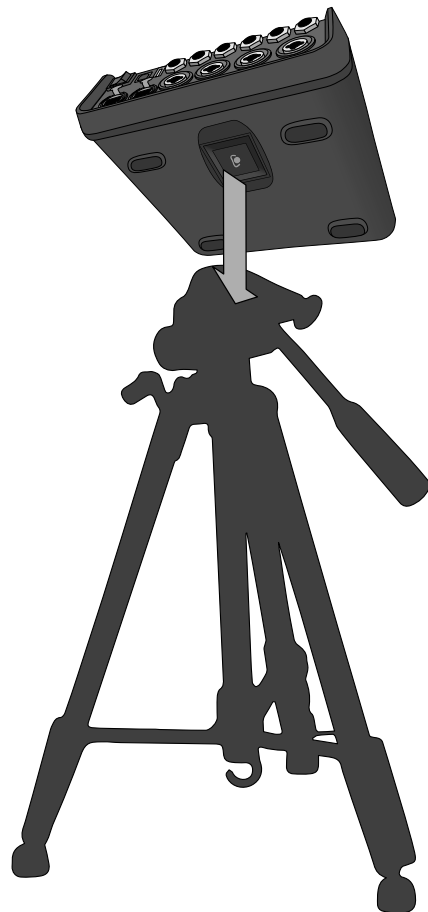
Figure 8. Mounting T4S to tripod stand using bracket
