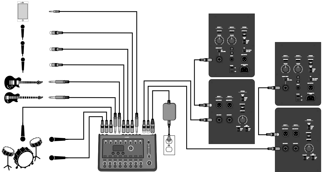
Figure 18. Example setup for Drums and Bass
