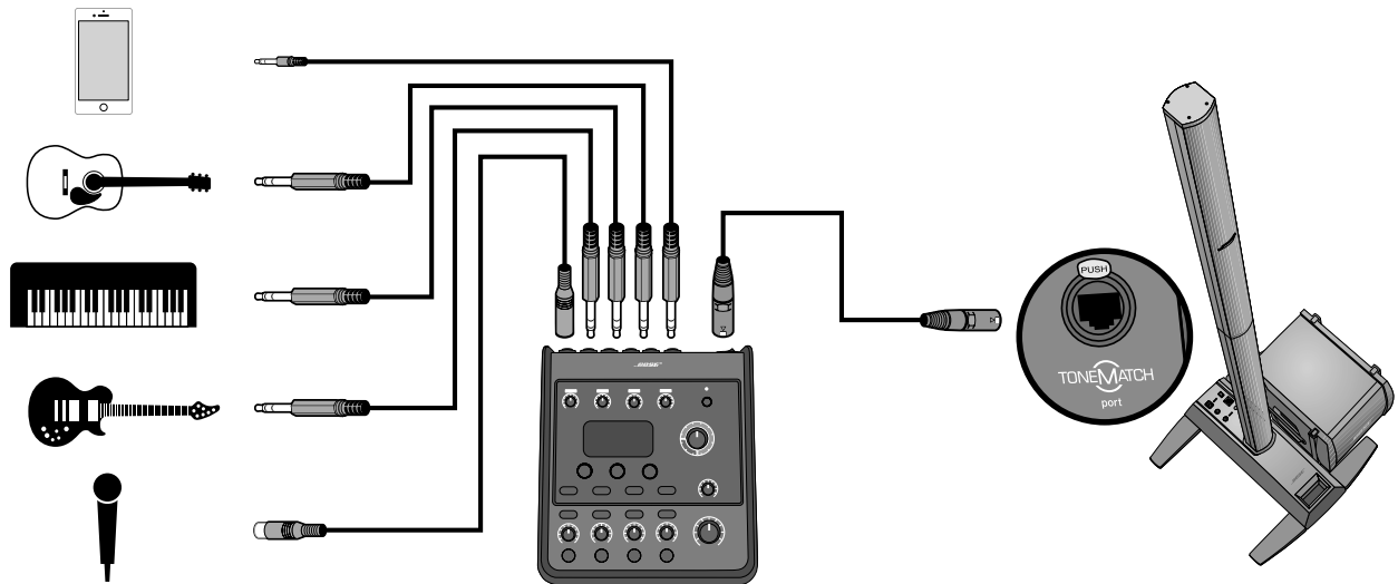
Figure 16. Example setup for Singer/Songwriter
