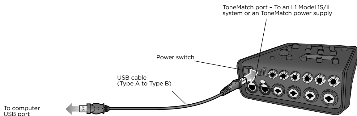
Figure 12. T4S-to-USB connection
