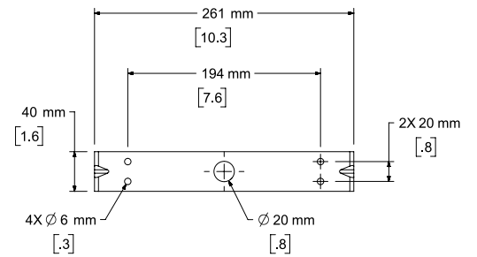
Rear View BRACKET ONLY
