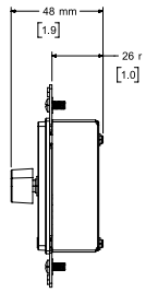
RIGHT VIEW DIMENSIONS APPLY TO BOTH SIDES
