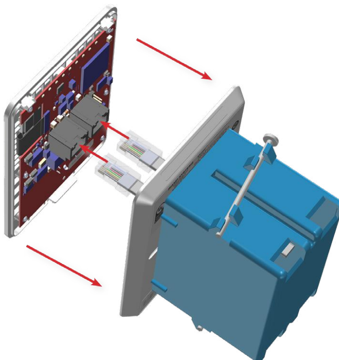
Figure 5. Connect Ethernet Cables
