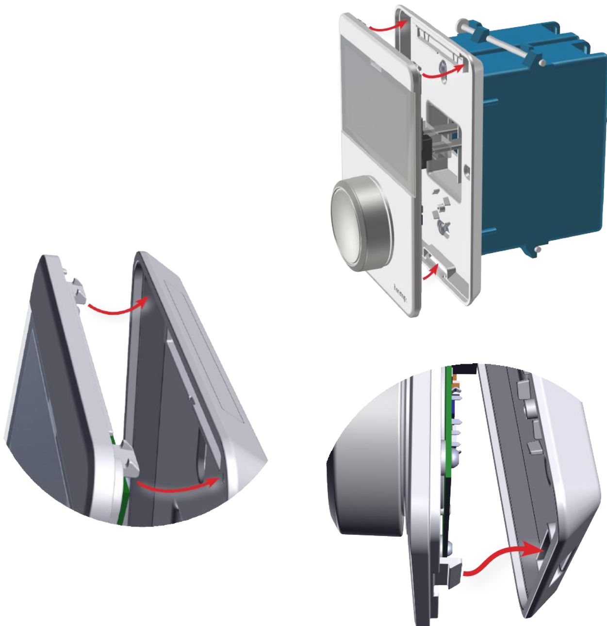
Figure 6. Clip Installation
