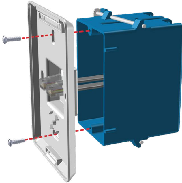
Figure 4. Back Plate Installation
