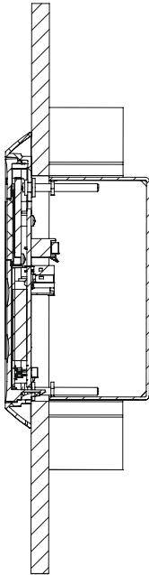
Mounting using a Raco 254 box
