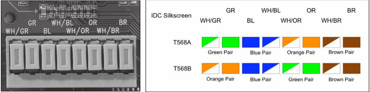
Insulation Displacement Connector (IDC)
