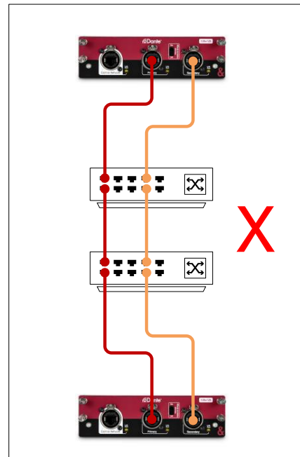
An incorrectly configured redundant Dante connection with shared network hardware for the Primary and Secondary connections
