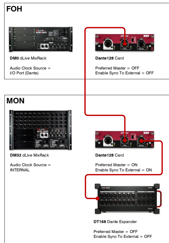
An example of a correctly configured Dante clock setup in a FoH/MON system
