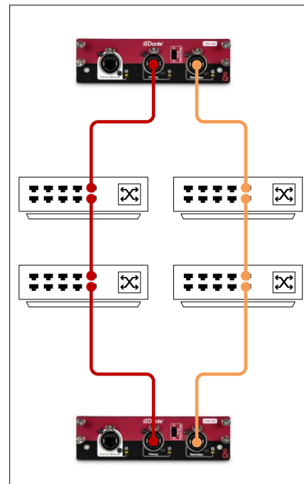
A correctly configured redundant Dante connection with discrete network hardware for both the Primary and Secondary connections
