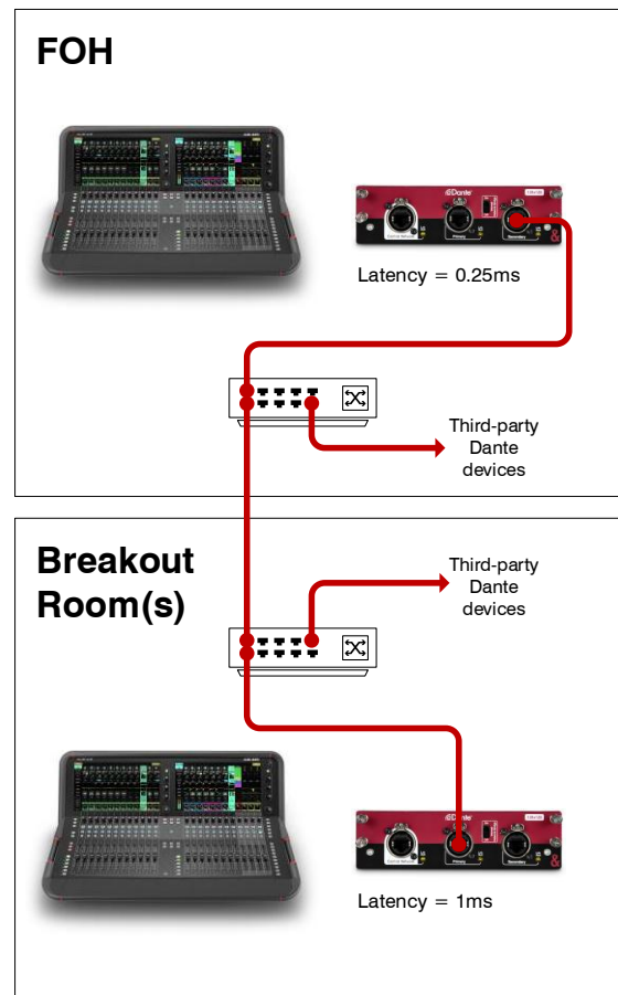
A basic Dante network with mixed latencies
